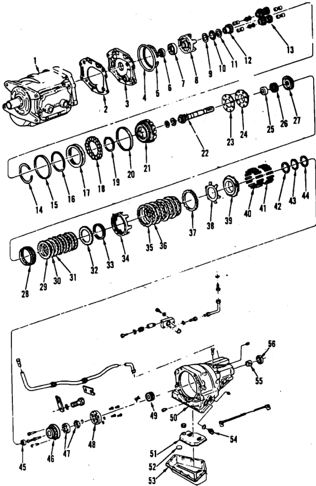
4 SPEED OVERDRIVE UNIT
